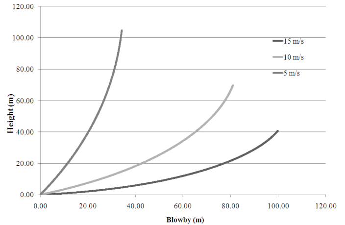
Fig. 3. Tether profiles for various wind speeds from the mooring point
