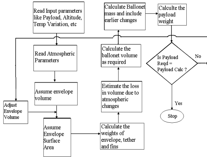
Fig. 2. Flow Chart of the aerostat design methodology [5]
