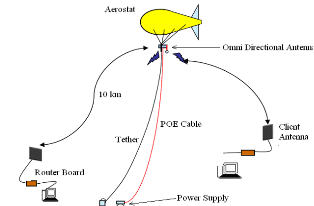
Fig. 1. Conceptual Sketch of the overall system
