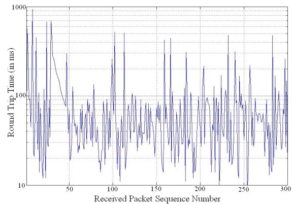
Fig. 6. Round Trip Time as a function of Received Packet Sequence Number. The graph shows the ping statistics for packet numbers 0 to 300 sent over 7 Kms link between BS and Client.
