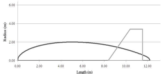
Fig. 4. Geometrical Output obtained from the aerostat design methodology
