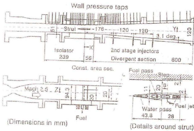
Fig.1 Schematic of the Combustor with the Strut
