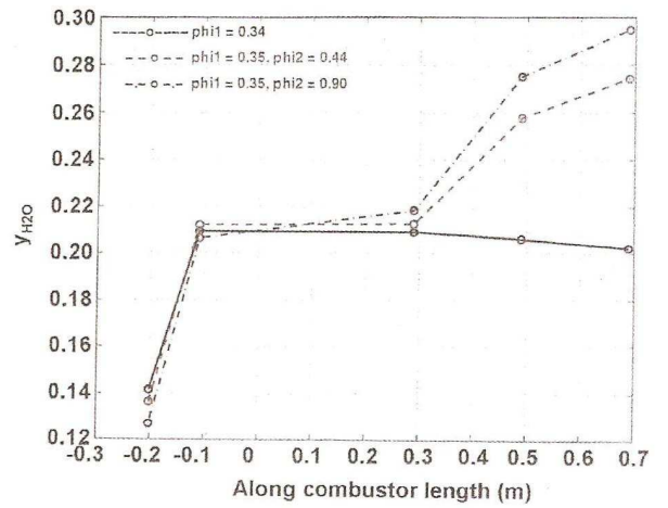
Fig.18 Axial Distribution of Area Averaged Water Mass Fraction for the Reacting Cases
