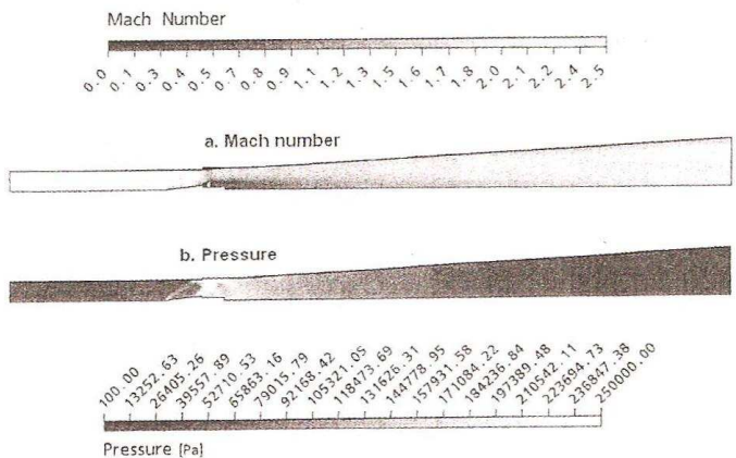
Fig.7 Flow Variables in the Symmetry Plane for Reacting Case with Strut Injection ( \phi_1=0.34 ) (a) Mach Number, (b) Pressure
