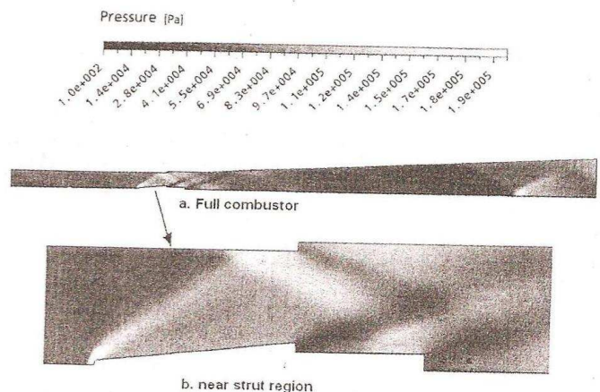
Fig.4 Pressure Distribution in the Symmetry Plane for Non Reacting Case (a) Full combustor, (b) Near Strut Region
